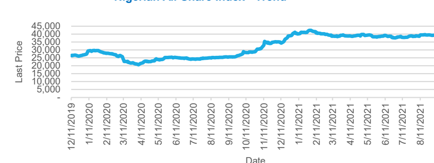
Nigerian All Share Index - Trend
